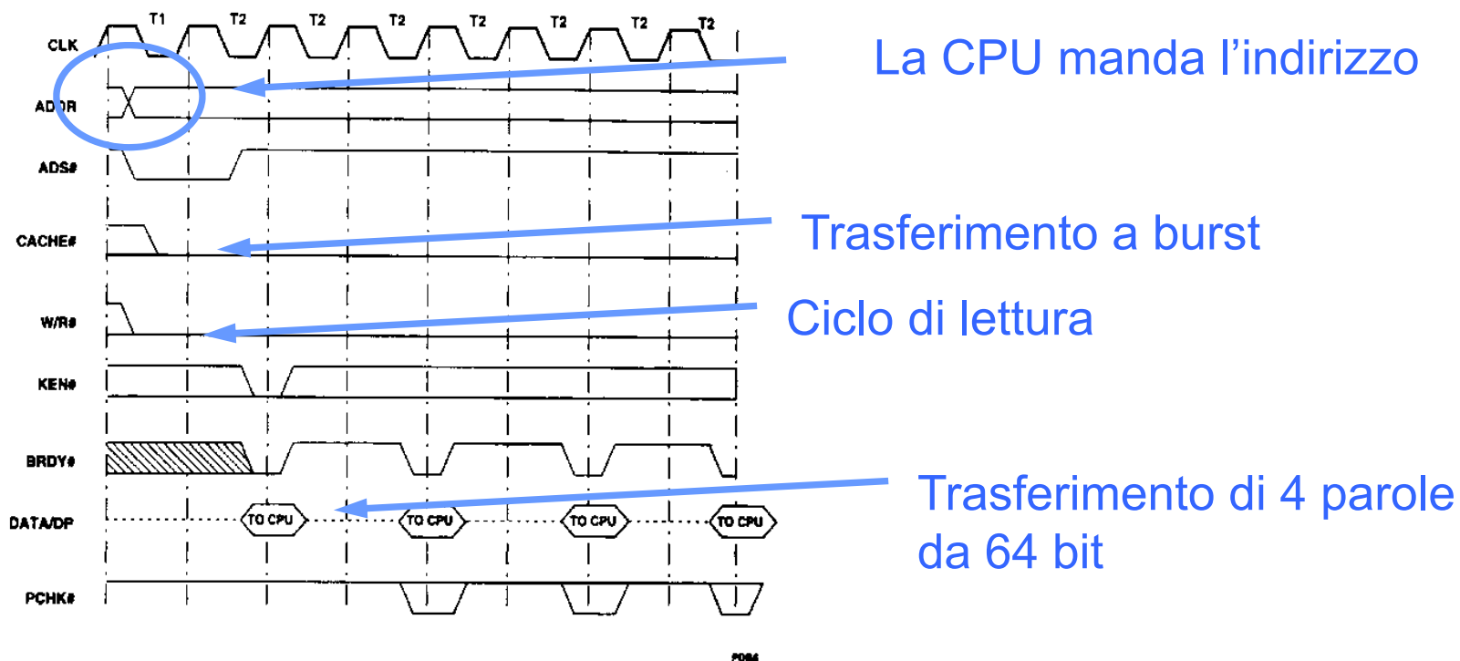
Figure 6-9. Slow Burst Read Cycle
